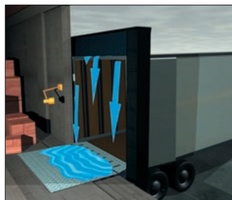
Ordinary head curtains cannot prevent the "Funnel Effect" when trailers approach down a decline during rain.
